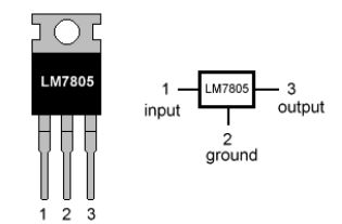
LM7805 PINOUT DIAGRAM
